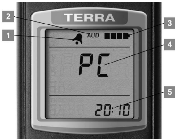
Figure 27 – LCD of the dosimeter (Bluetooth radio channel control mode)
