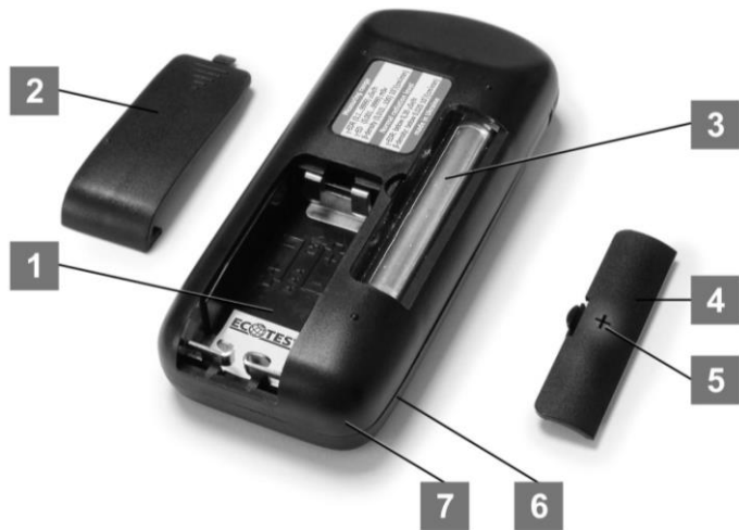
Figure 2 - External view of the dosimeter (bottom view)
