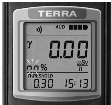
Figure 6 – LCD of the dosimeter (measurement restart)
