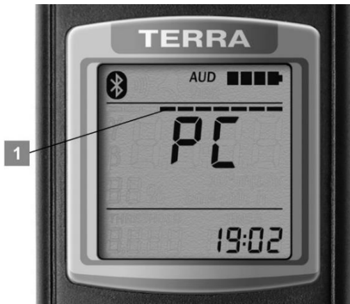
Figure 28 – LCD of the dosimeter (Bluetooth radio channel control mode)
